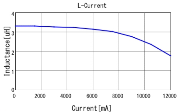
■ 1217AS-H-3R3N L-Current 20degC
